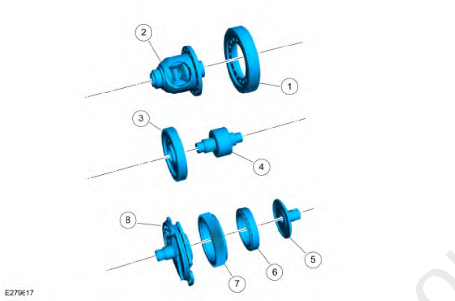
Final Drive Component Exploded View
